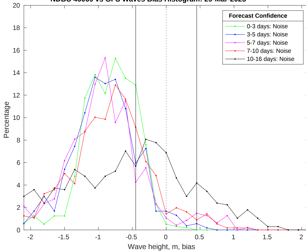
NDBC 46069 vs GFS Waves Bias Histogram: 29-Mar-2025
