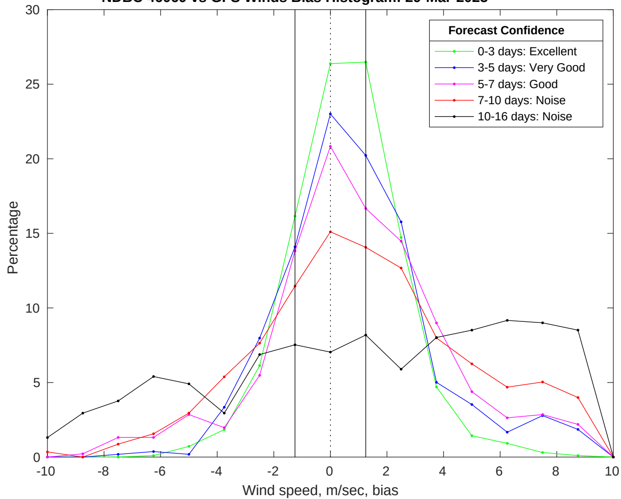
NDBC 46069 vs GFS Winds Bias Histogram: 29-Mar-2025
