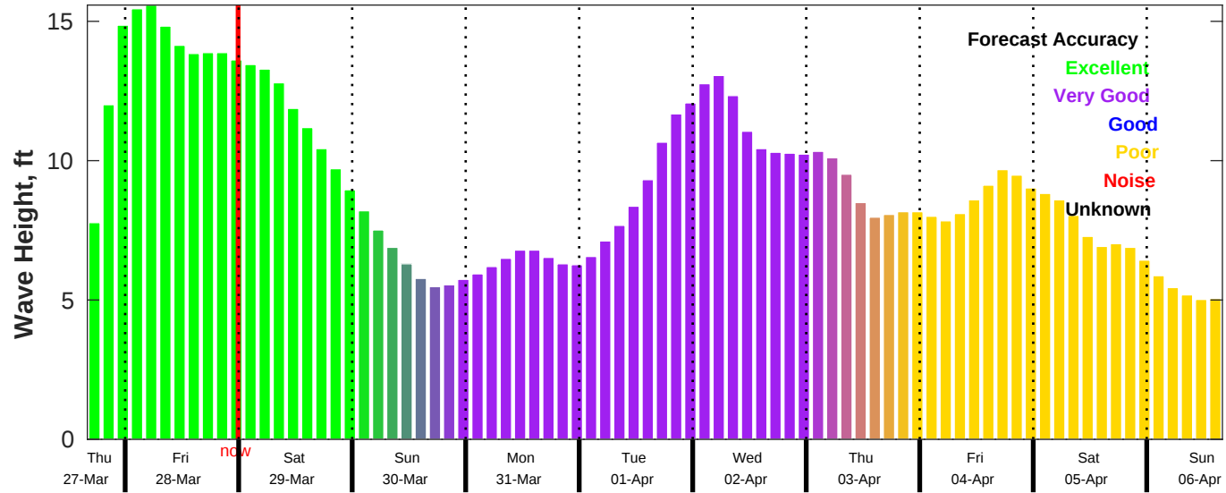
CEMS Wave Forecast for NDBC 46069 from 27-Mar-2025 16:00:00 to 06-Apr-2025 16:00:00
