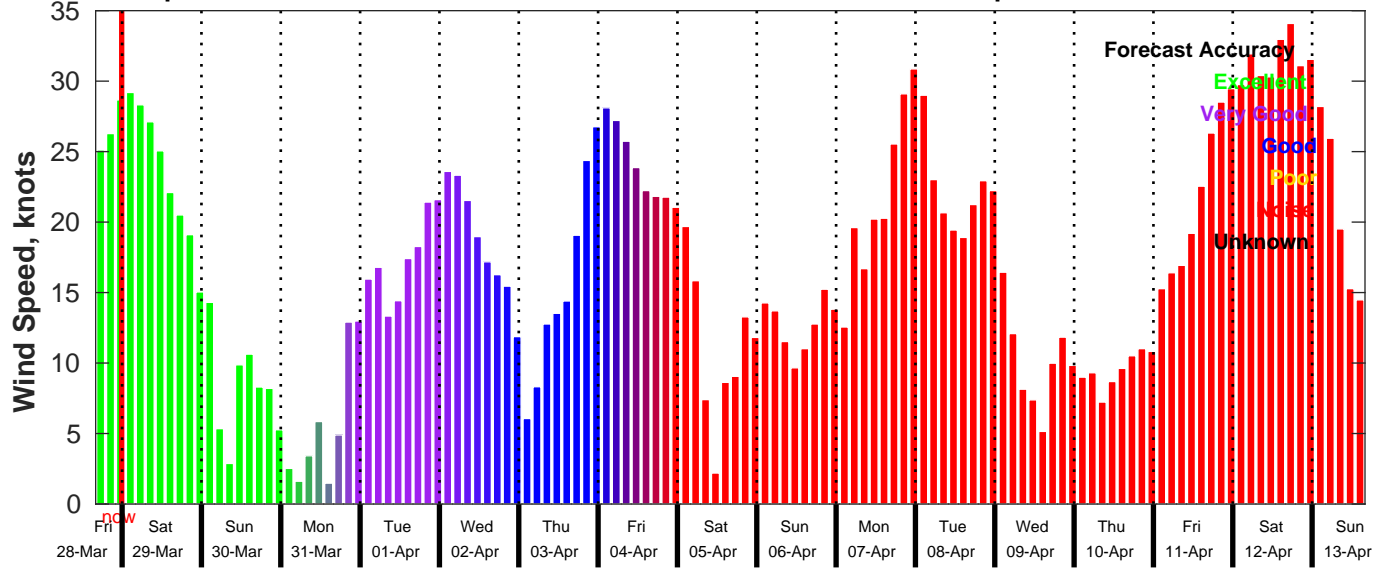
GFS Wind Speed Forecast for NDBC 46069 from 28-Mar-2025 16:00:00 to 13-Apr-2025 16:00:00
