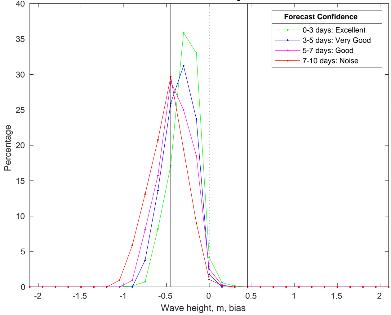
NDBC 51209 vs CMEMS Waves Bias Histogram: 29-Mar-2025
