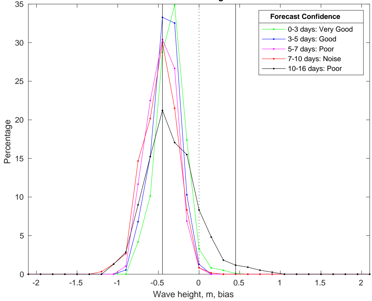
NDBC 51209 vs GFS Waves Bias Histogram: 29-Mar-2025
