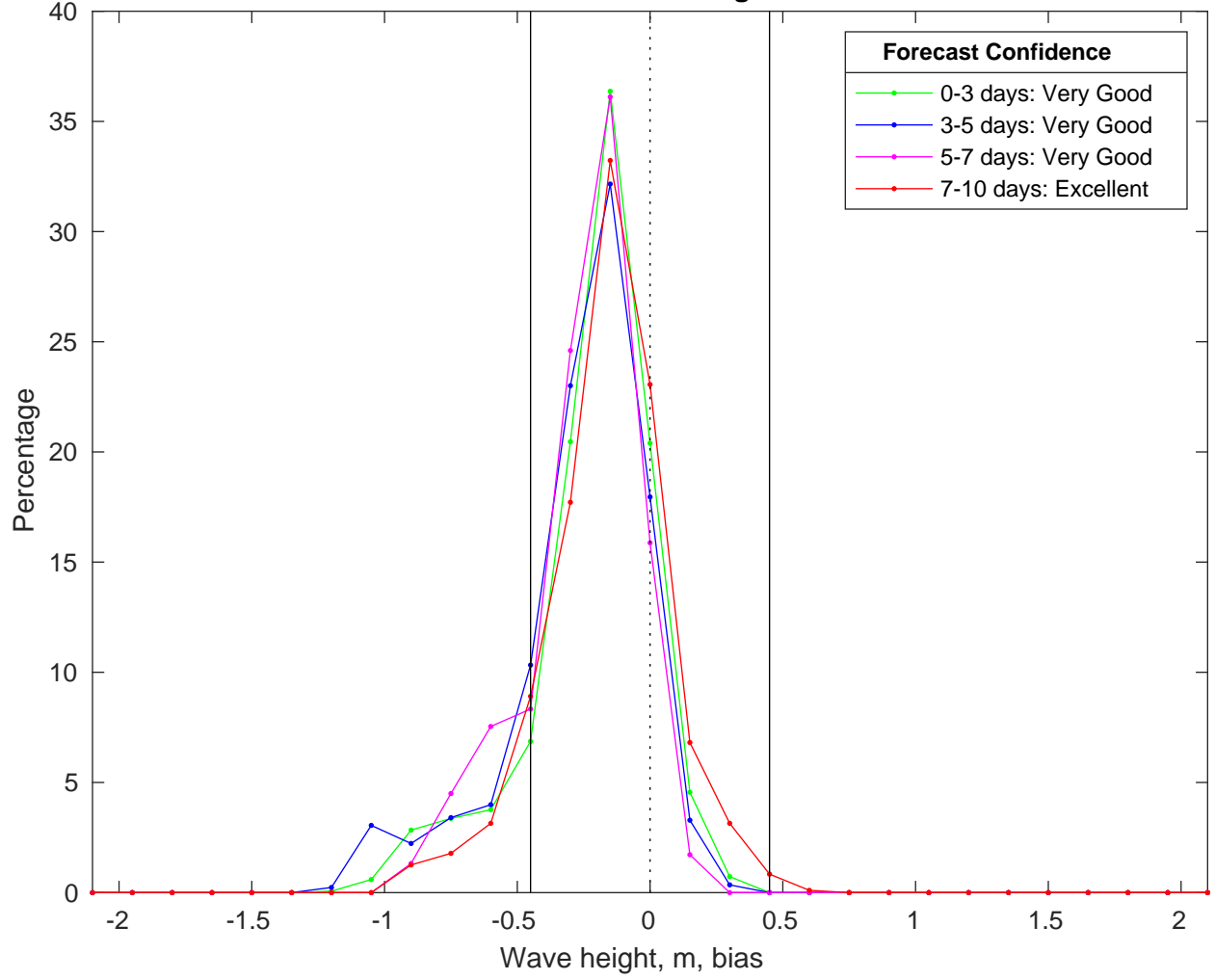
NDBC 52211 vs CMEMS Waves Bias Histogram: 29-Mar-2025
