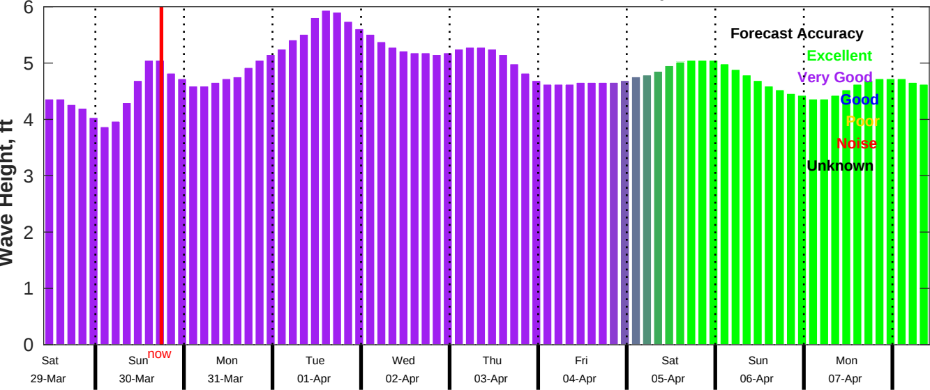
CMEMS Wave Forecast for NDBC 52211 from 28-Mar-2025 10:00:00 to 07-Apr-2025 10:00:00
