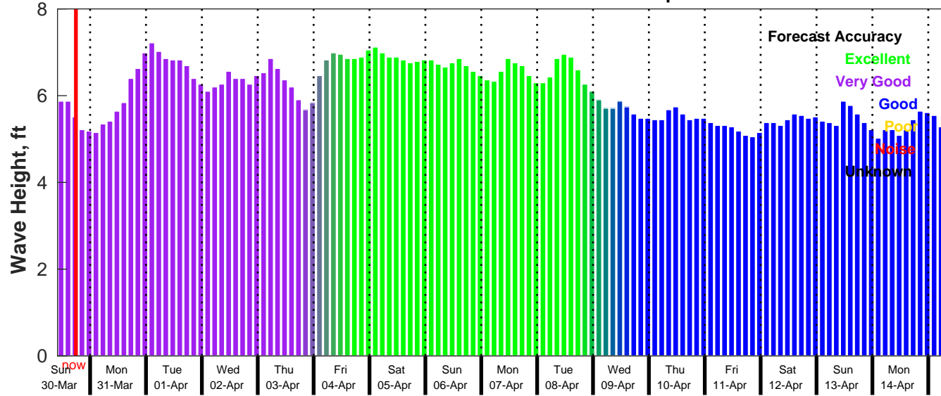
GFS Wave Forecast for NDBC 52211 from 29-Mar-2025 10:00:00 to 14-Apr-2025 10:00:00
