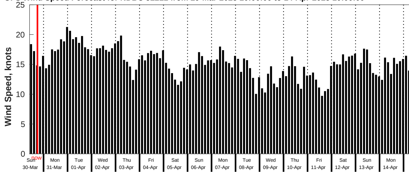
GFS Wind Speed Forecast for NDBC 52211 from 29-Mar-2025 10:00:00 to 14-Apr-2025 10:00:00
