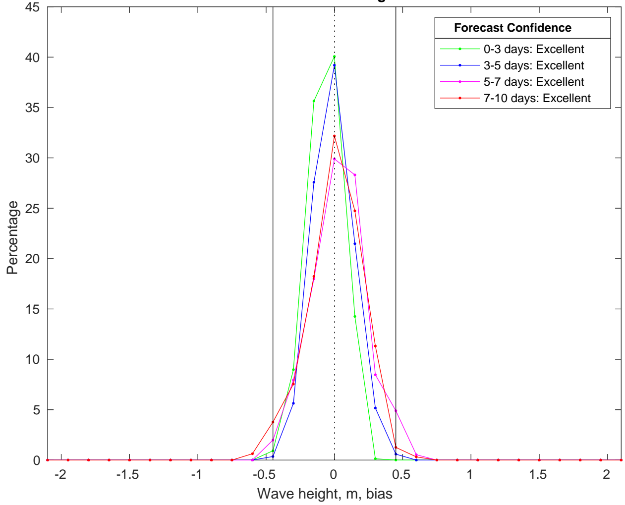
NDBC 52212 vs CMEMS Waves Bias Histogram: 29-Mar-2025
