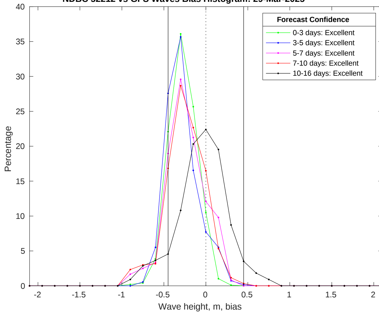
NDBC 52212 vs GFS Waves Bias Histogram: 29-Mar-2025
