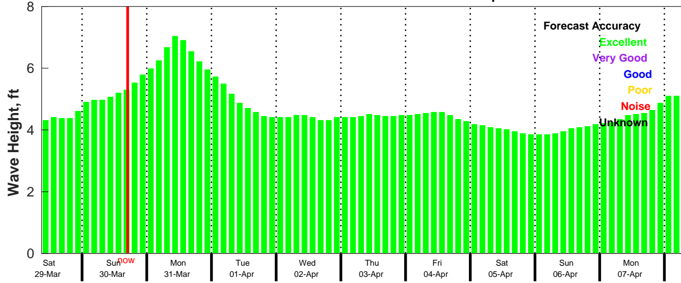
CMEMS Wave Forecast for NDBC 52212 from 28-Mar-2025 09:00:00 to 07-Apr-2025 09:00:00
