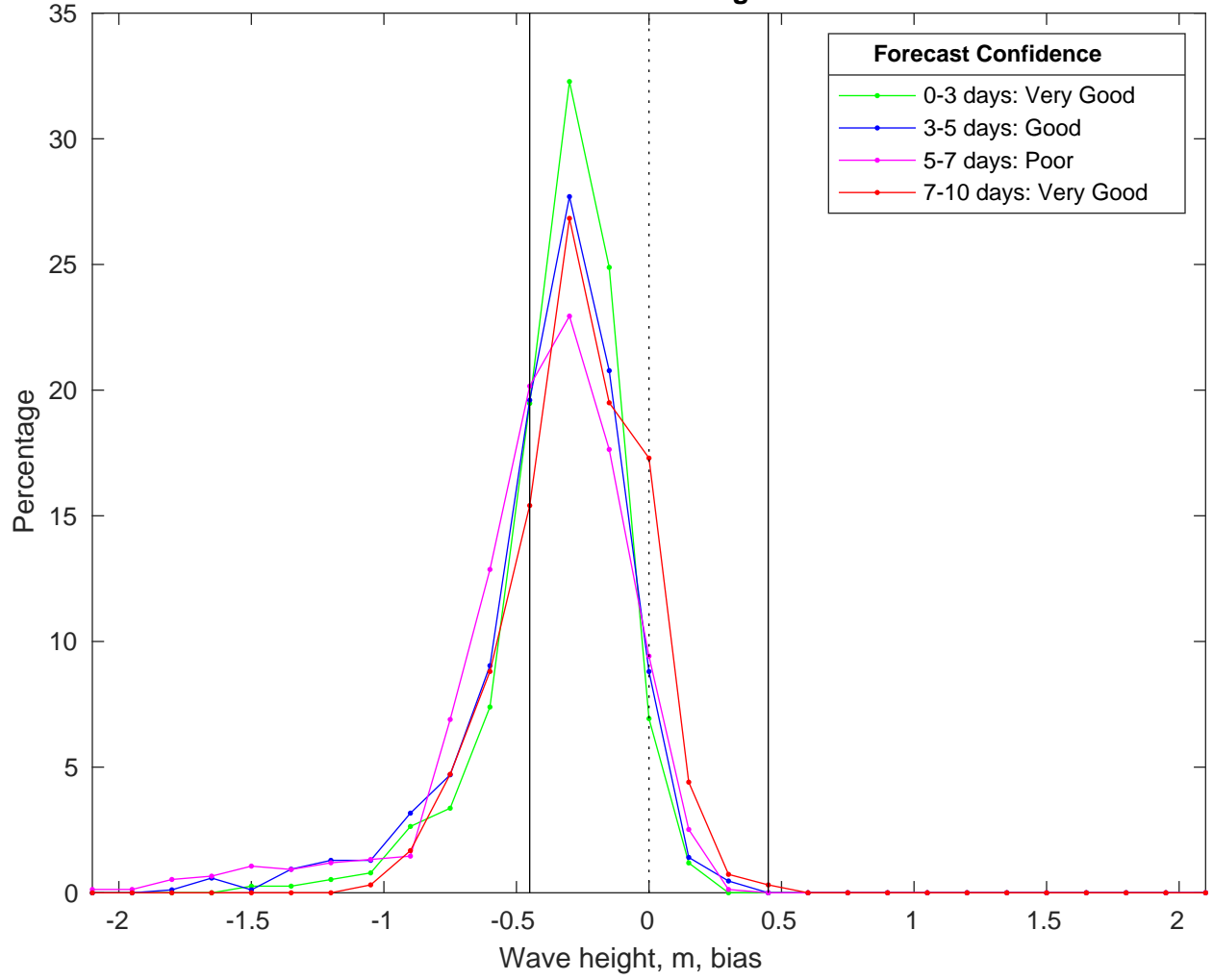
NDBC 52213 vs CMEMS Waves Bias Histogram: 29-Mar-2025
