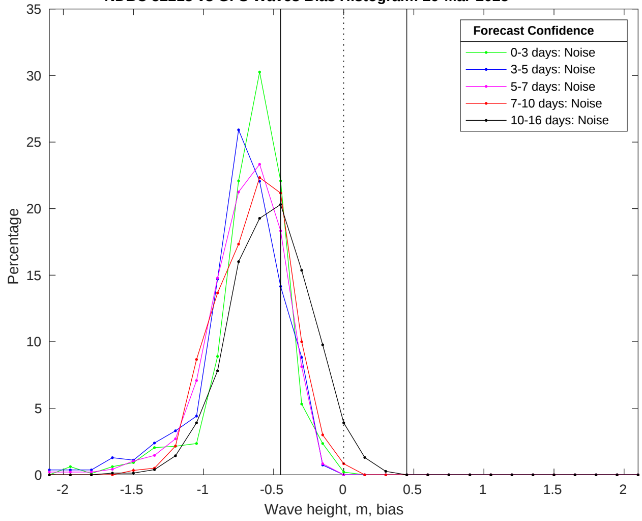
NDBC 52213 vs GFS Waves Bias Histogram: 29-Mar-2025
