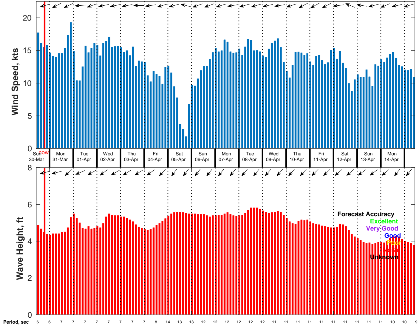
Wind & Wave Forecast for NDBC 52213 from 29-Mar-2025 11:00:00 to 14-Apr-2025 11:00:00
