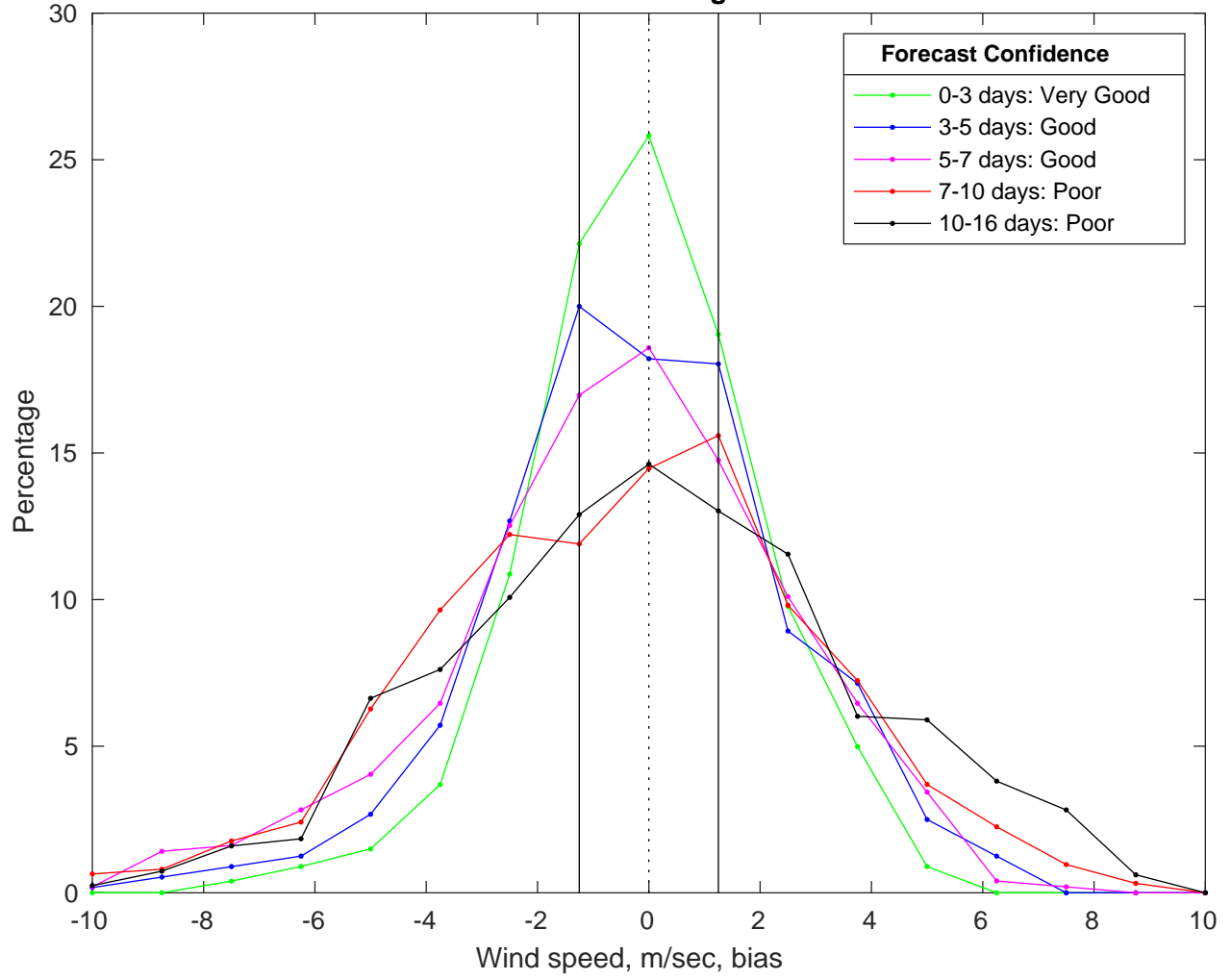
NDBC 41004 vs GFS Winds Bias Histogram: 30-Mar-2025
