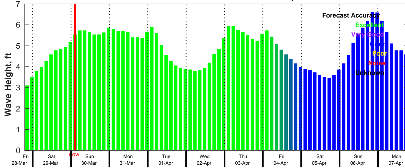
CMEMS Wave Forecast for NDBC 41004 from 28-Mar-2025 19:00:00 to 07-Apr-2025 19:00:00
