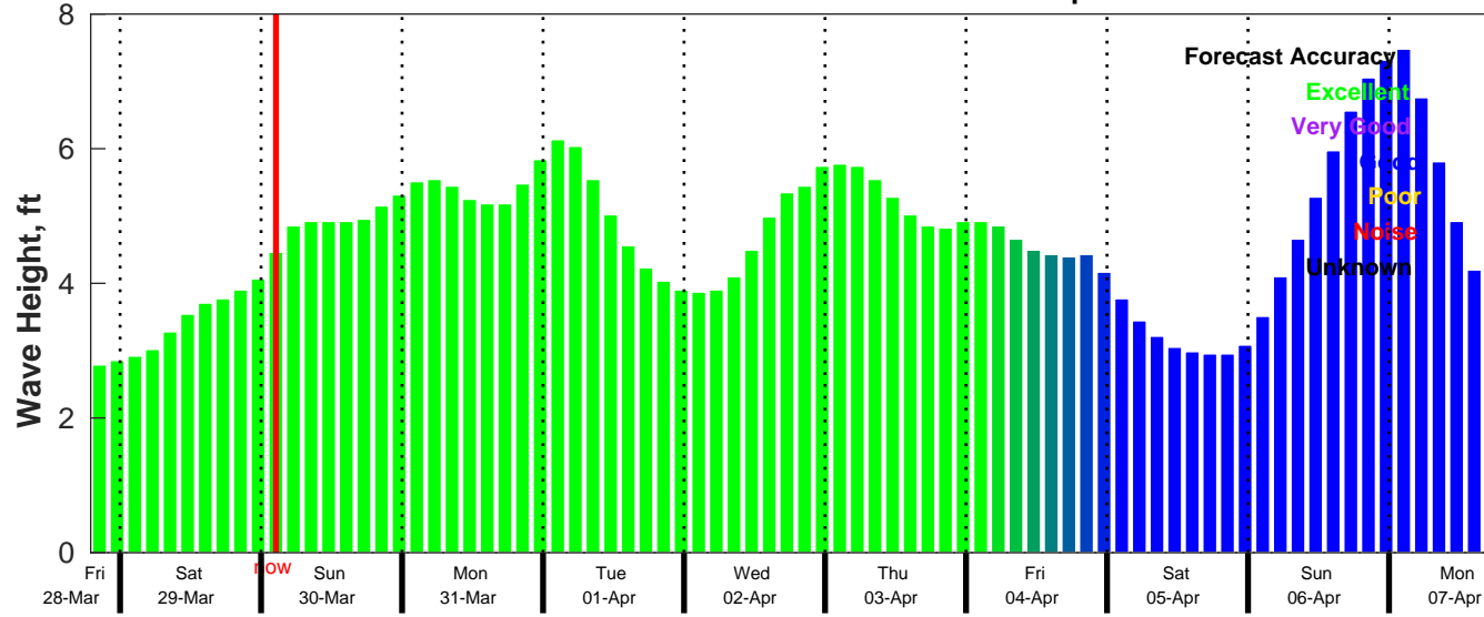
CMEMS Wave Forecast for NDBC 41013 from 28-Mar-2025 19:00:00 to 07-Apr-2025 19:00:00
