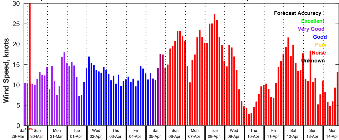
GFS Wind Speed Forecast for NDBC 41013 from 29-Mar-2025 19:00:00 to 14-Apr-2025 19:00:00
