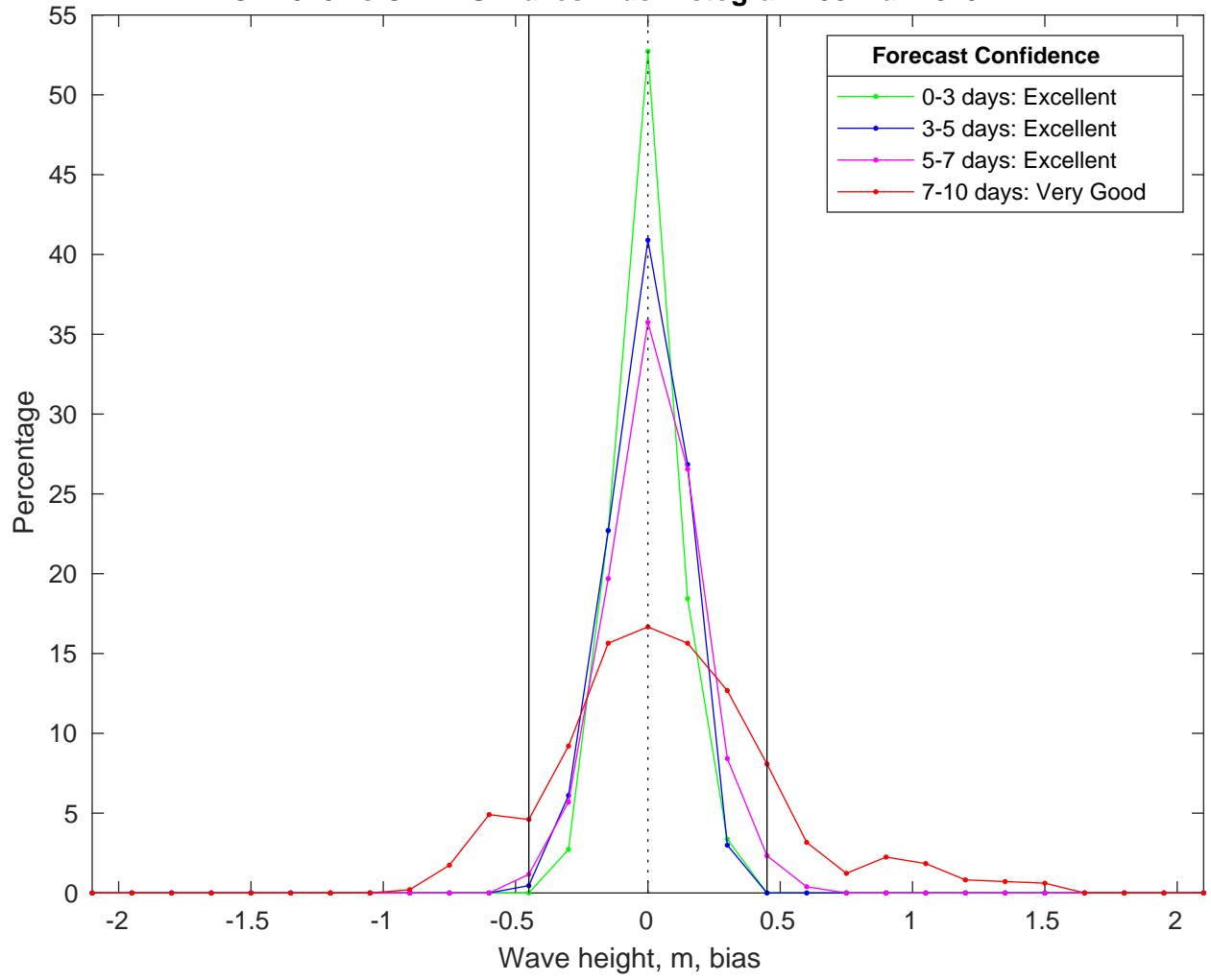
NDBC 41040 vs CMEMS Waves Bias Histogram: 30-Mar-2025
