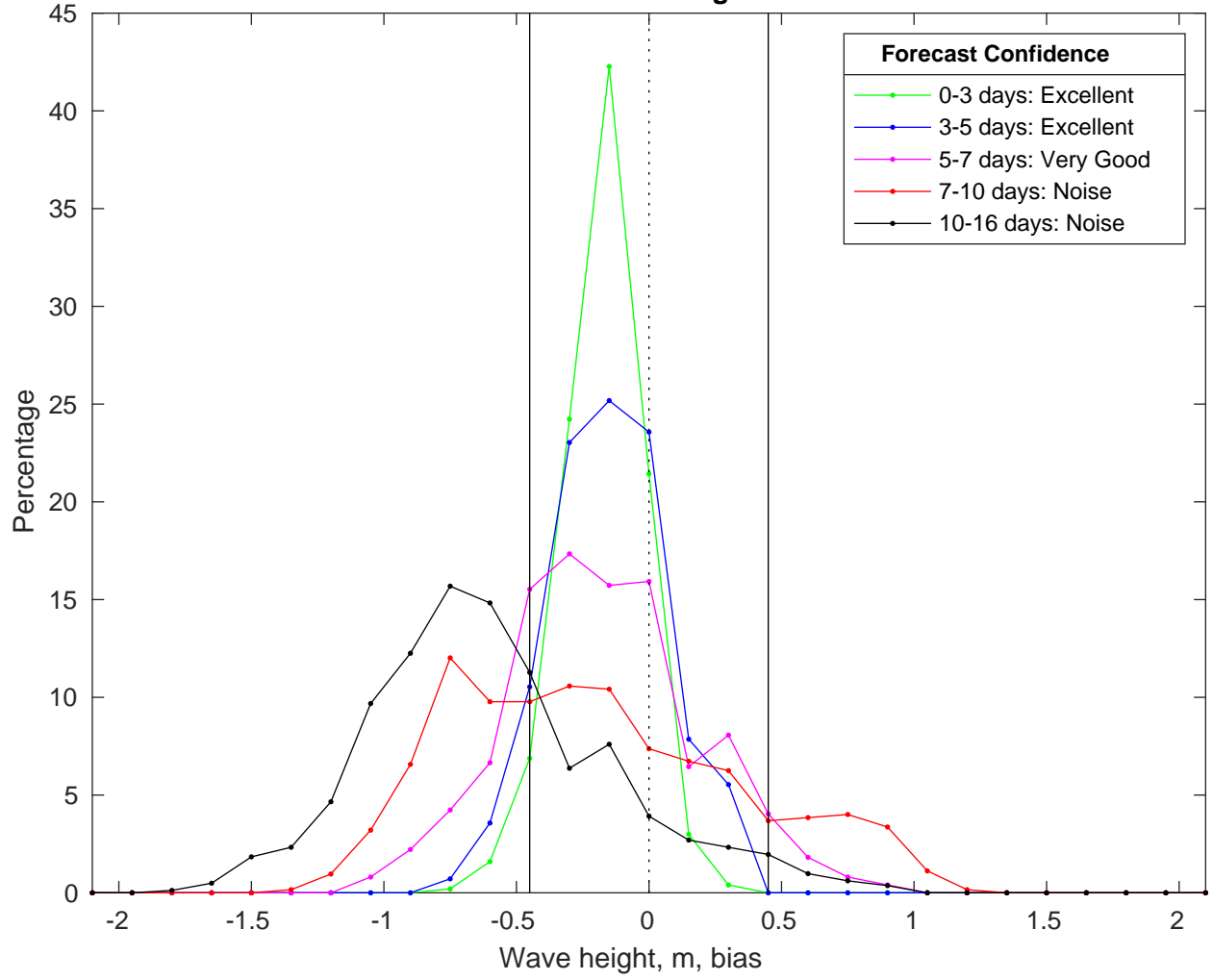
NDBC 41040 vs GFS Waves Bias Histogram: 30-Mar-2025
