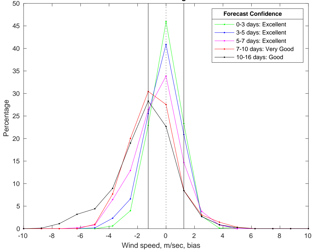
NDBC 41040 vs GFS Winds Bias Histogram: 30-Mar-2025
