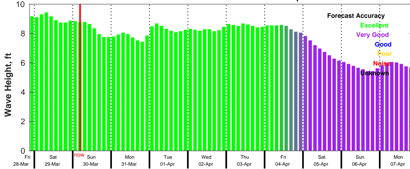
CMEMS Wave Forecast for NDBC 41040 from 28-Mar-2025 21:00:00 to 07-Apr-2025 21:00:00
