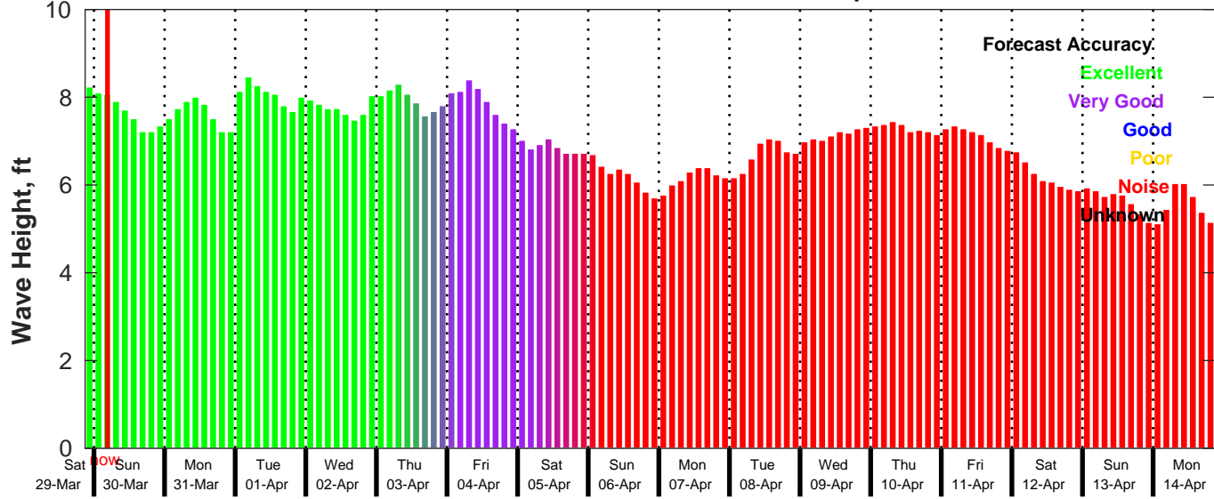
GFS Wave Forecast for NDBC 41040 from 29-Mar-2025 21:00:00 to 14-Apr-2025 21:00:00
