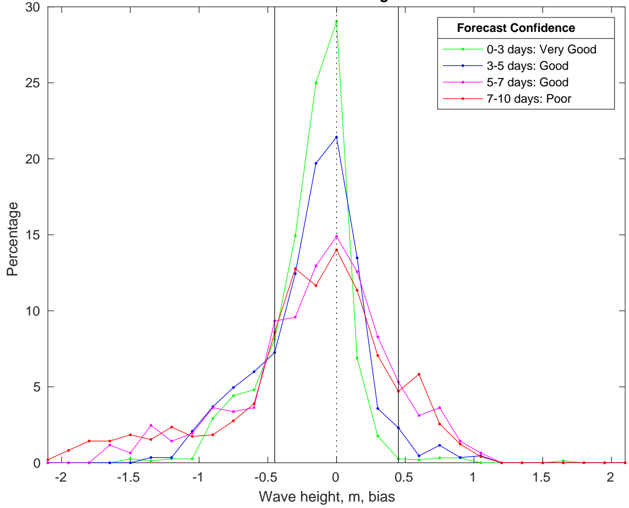
NDBC 42019 vs CMEMS Waves Bias Histogram: 30-Mar-2025
