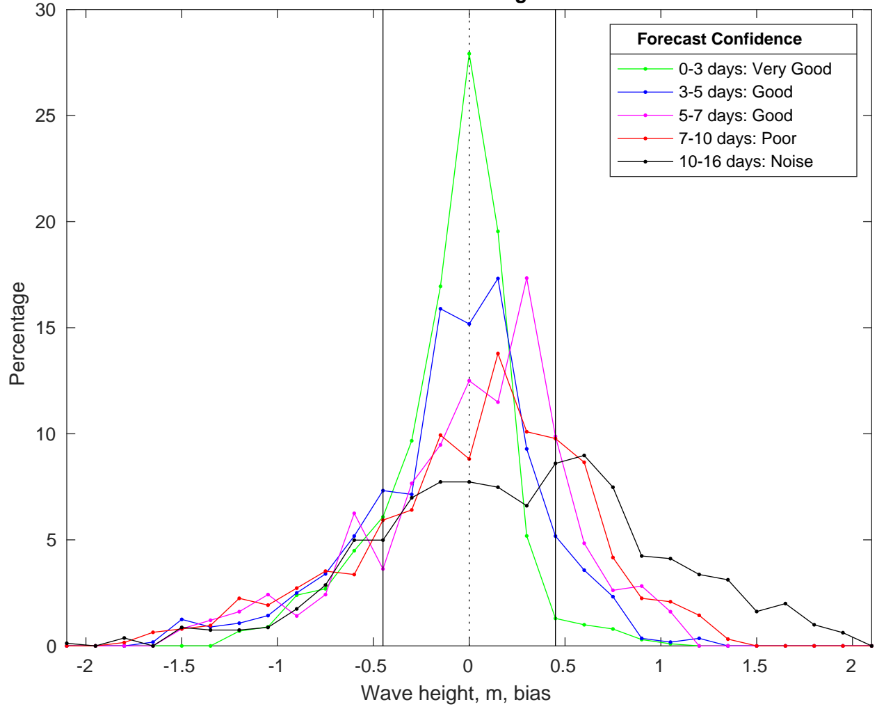
NDBC 42019 vs GFS Waves Bias Histogram: 30-Mar-2025
