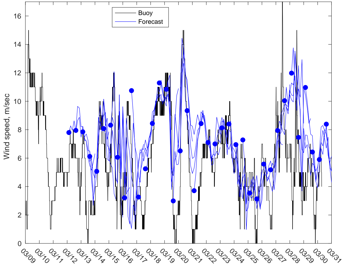
NDBC 42019 vs GFS Winds: 3 to 5 day forecast
