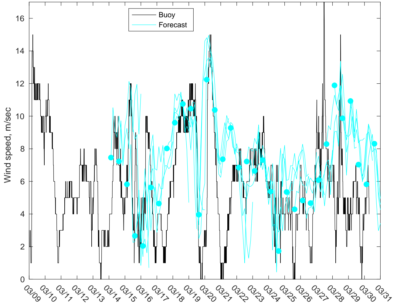
NDBC 42019 vs GFS Winds: 5 to 7 day forecast
