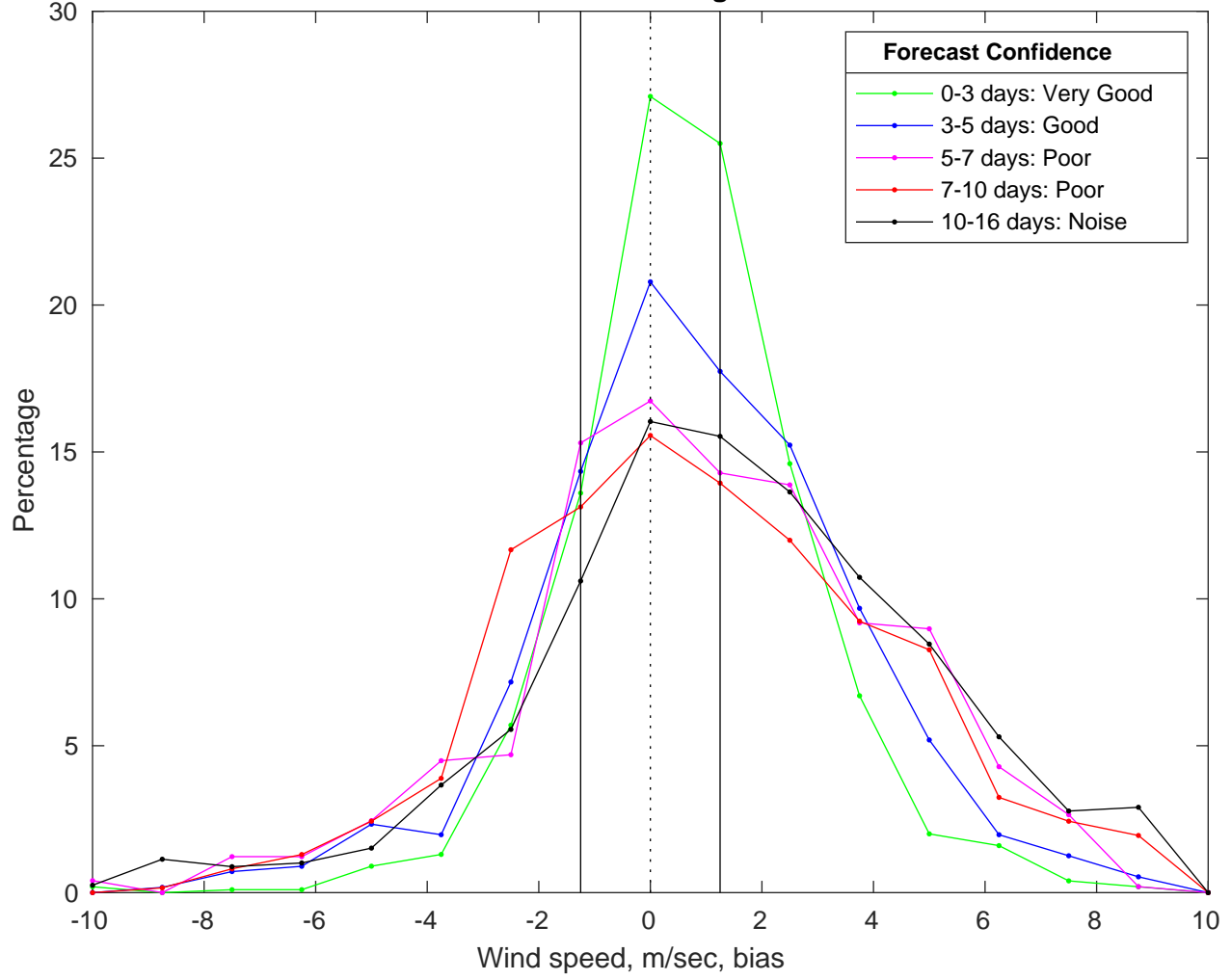
NDBC 42019 vs GFS Winds Bias Histogram: 30-Mar-2025
