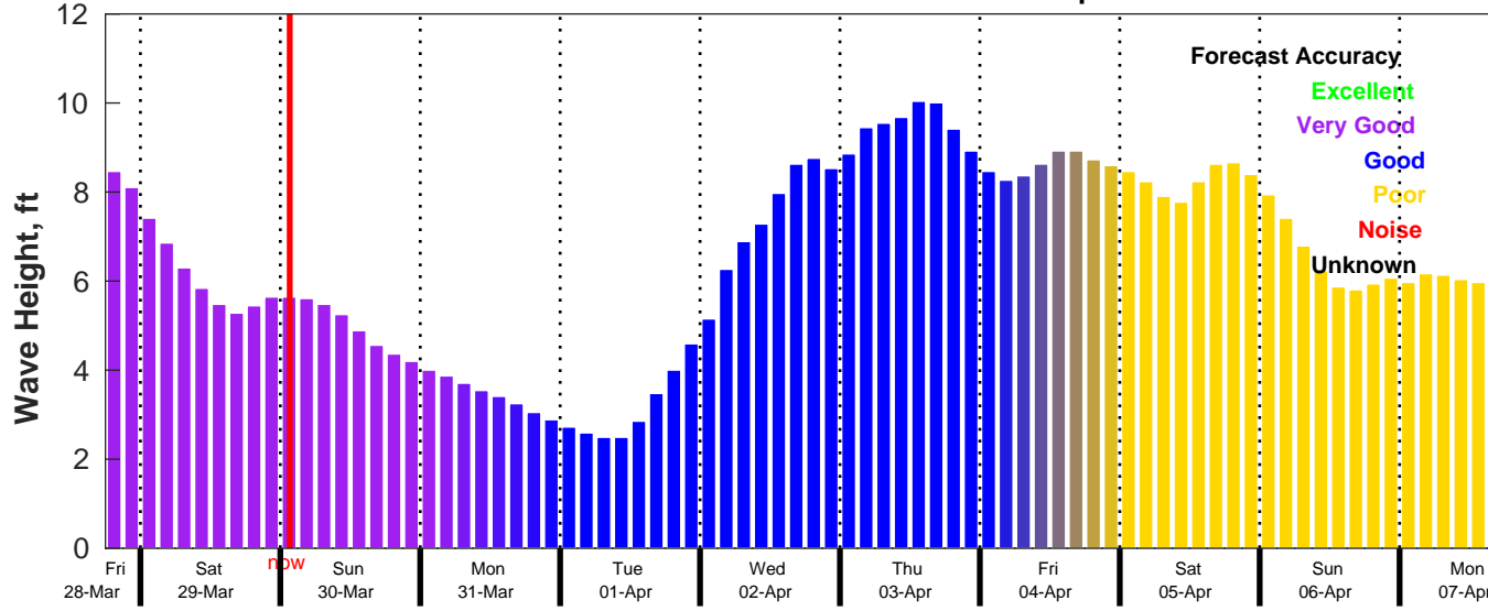
CMEMS Wave Forecast for NDBC 42019 from 28-Mar-2025 18:00:00 to 07-Apr-2025 18:00:00
