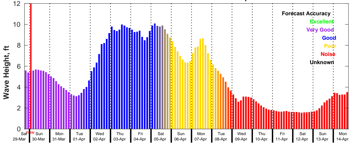
GFS Wave Forecast for NDBC 42019 from 29-Mar-2025 18:00:00 to 14-Apr-2025 18:00:00
