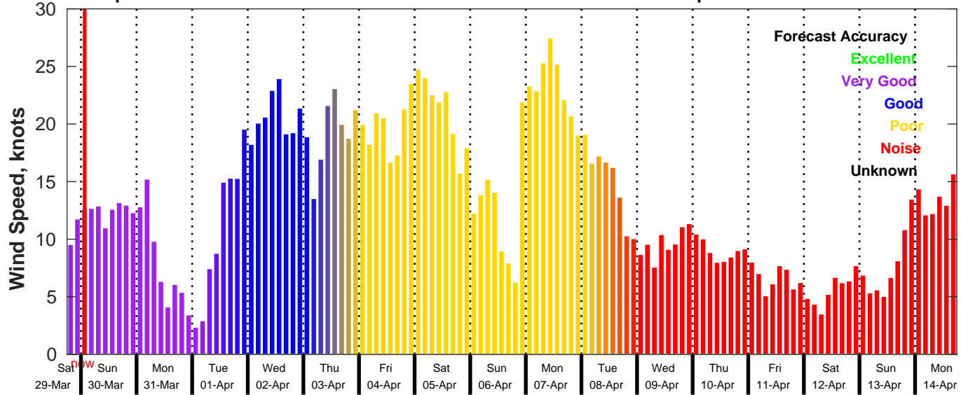
GFS Wind Speed Forecast for NDBC 42019 from 29-Mar-2025 18:00:00 to 14-Apr-2025 18:00:00
