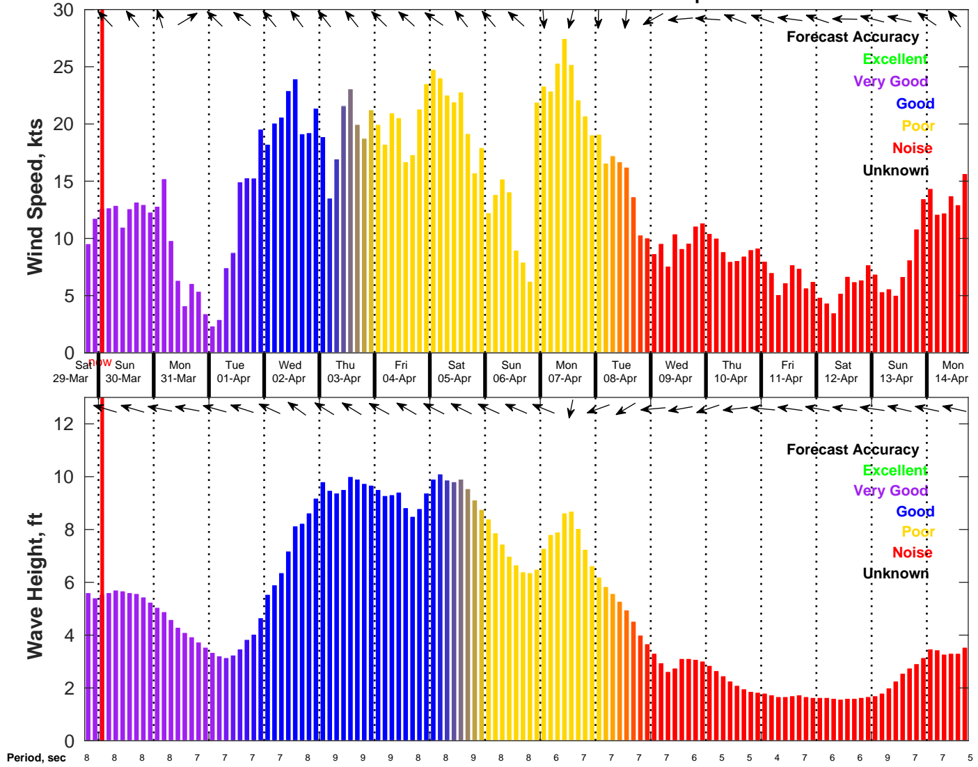
Wind & Wave Forecast for NDBC 42019 from 29-Mar-2025 18:00:00 to 14-Apr-2025 18:00:00
