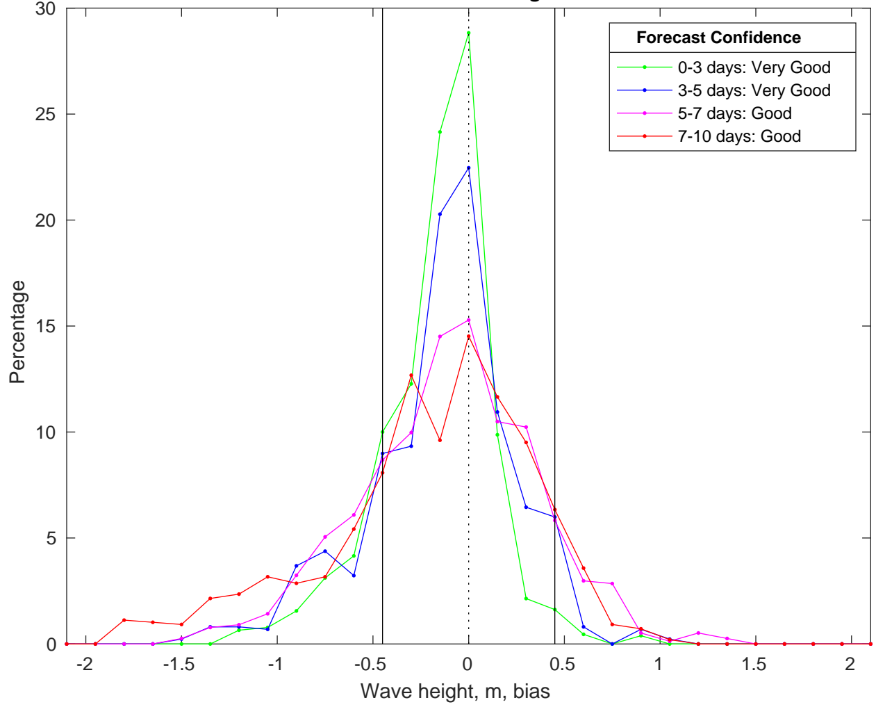
NDBC 42020 vs CMEMS Waves Bias Histogram: 30-Mar-2025
