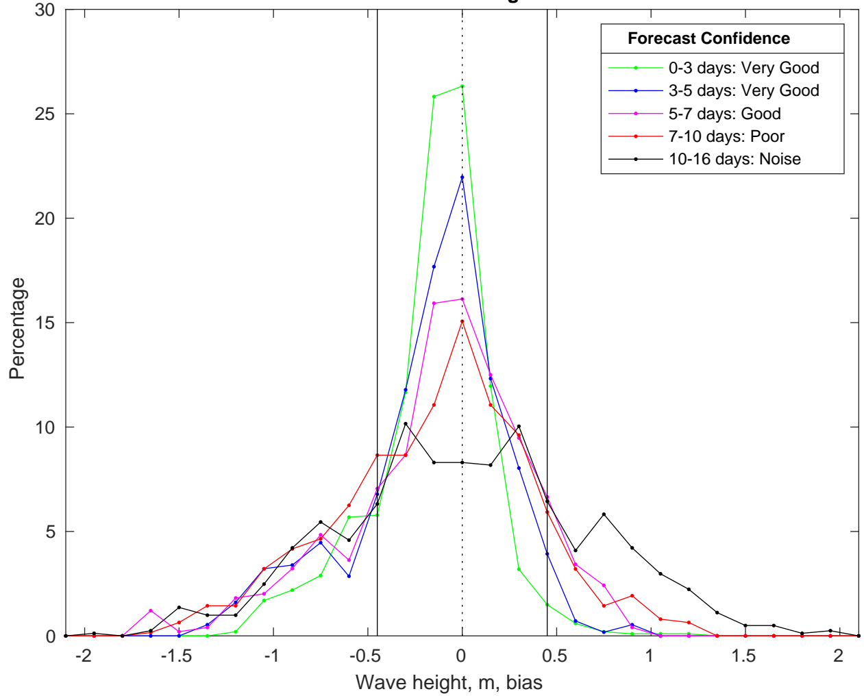
NDBC 42020 vs GFS Waves Bias Histogram: 30-Mar-2025
