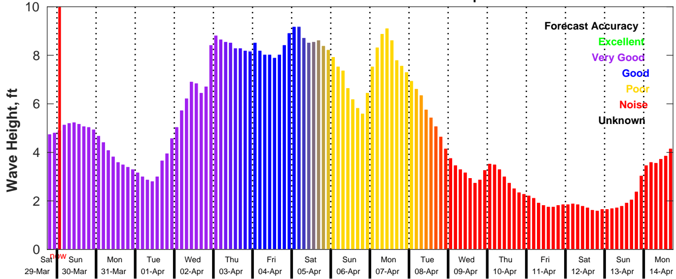
GFS Wave Forecast for NDBC 42020 from 29-Mar-2025 18:00:00 to 14-Apr-2025 18:00:00
