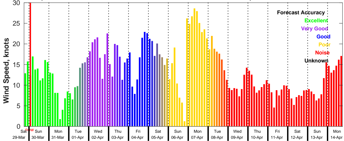
GFS Wind Speed Forecast for NDBC 42020 from 29-Mar-2025 18:00:00 to 14-Apr-2025 18:00:00
