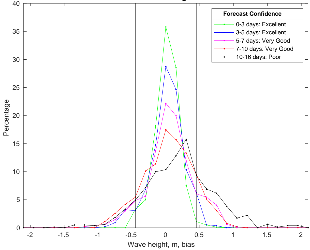
NDBC 42035 vs GFS Waves Bias Histogram: 30-Mar-2025
