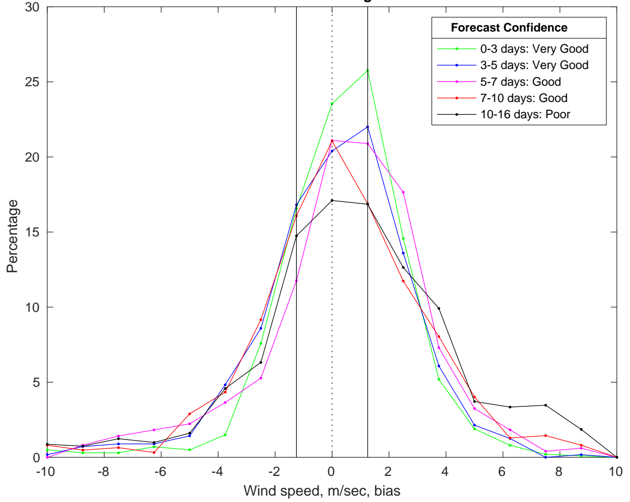
NDBC 42035 vs GFS Winds Bias Histogram: 30-Mar-2025
