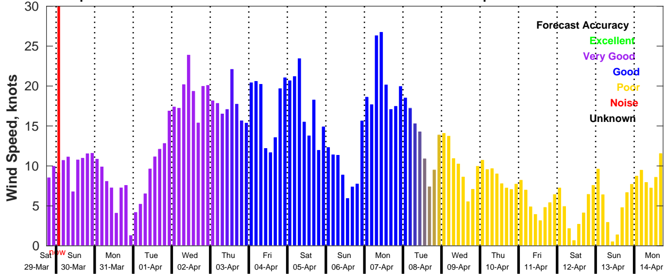
GFS Wind Speed Forecast for NDBC 42035 from 29-Mar-2025 18:00:00 to 14-Apr-2025 18:00:00
