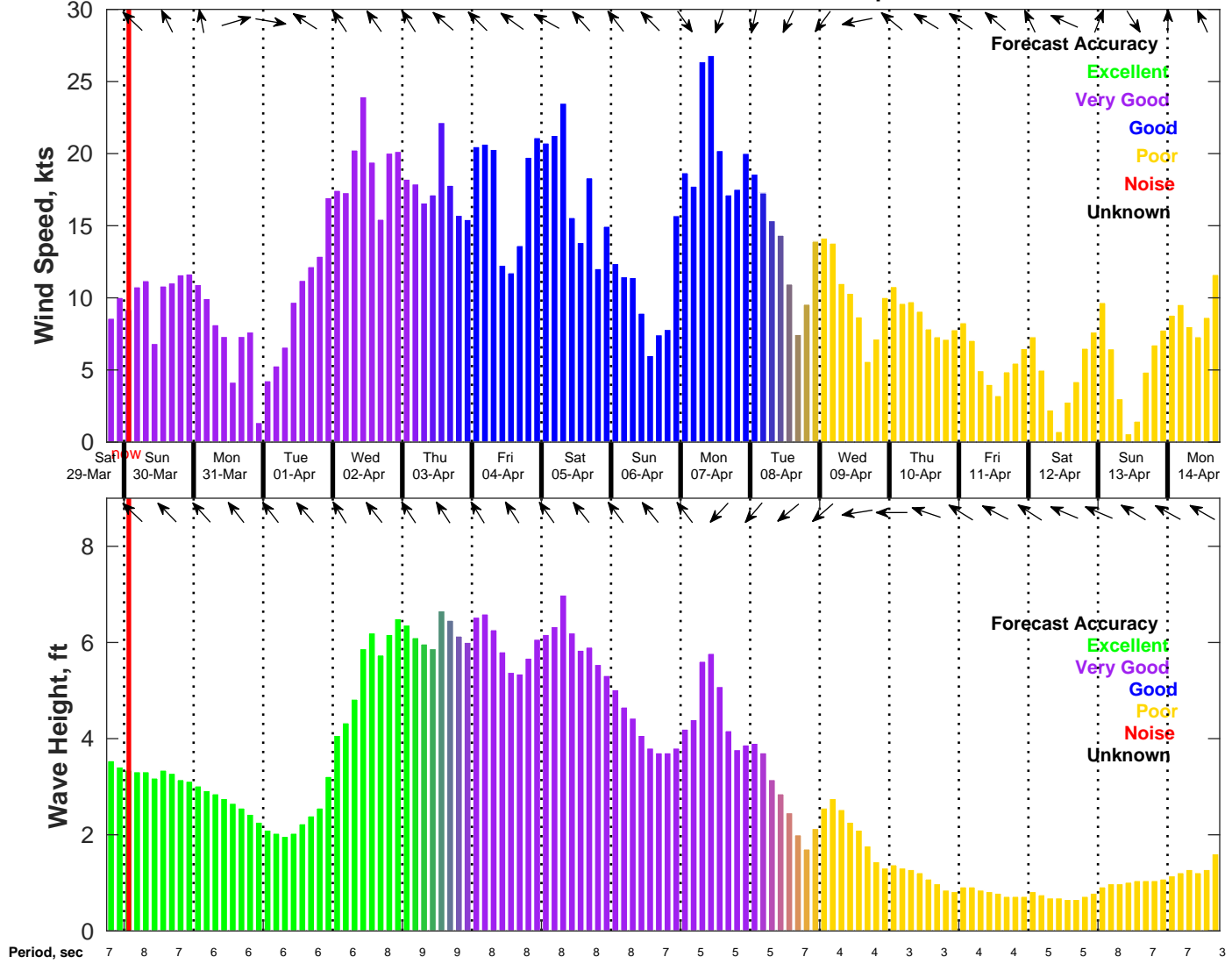
Wind & Wave Forecast for NDBC 42035 from 29-Mar-2025 18:00:00 to 14-Apr-2025 18:00:00
