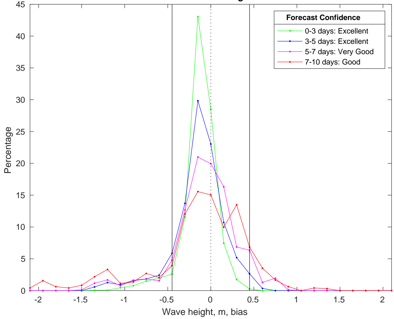
NDBC 42036 vs CMEMS Waves Bias Histogram: 30-Mar-2025
