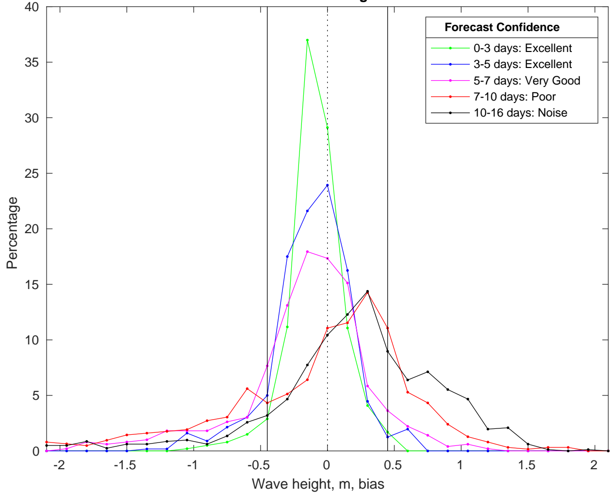
NDBC 42036 vs GFS Waves Bias Histogram: 30-Mar-2025
