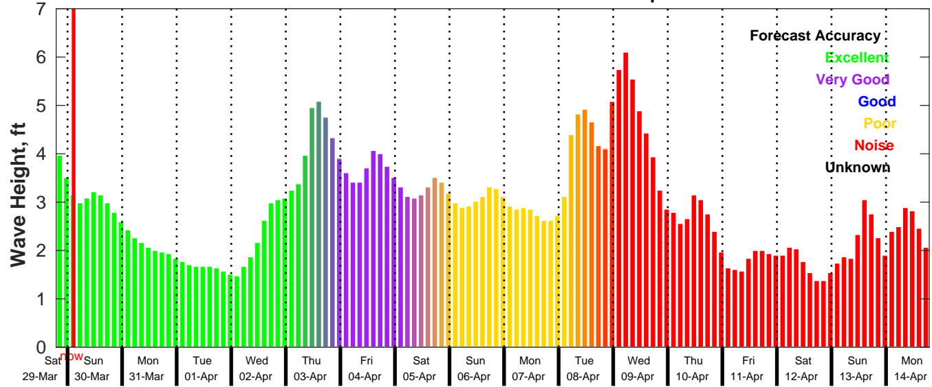
GFS Wave Forecast for NDBC 42036 from 29-Mar-2025 19:00:00 to 14-Apr-2025 19:00:00
