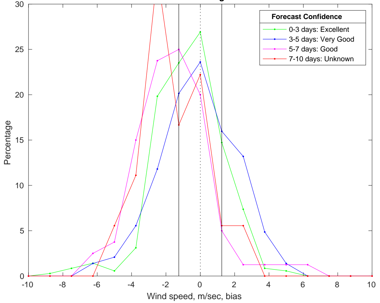
NDBC 42040 vs GFS Winds Bias Histogram: 30-Mar-2025
