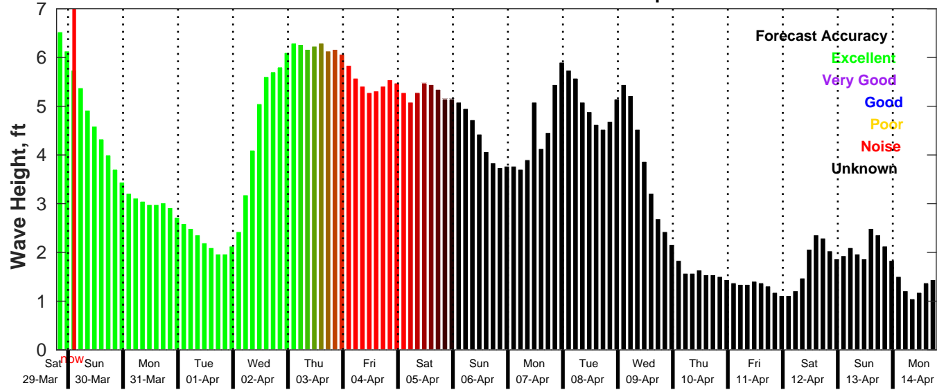
GFS Wave Forecast for NDBC 42040 from 29-Mar-2025 19:00:00 to 14-Apr-2025 19:00:00
