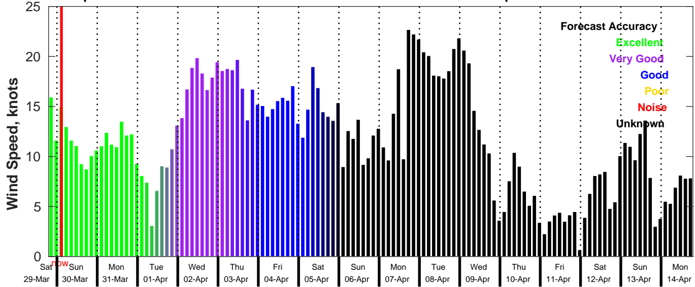
GFS Wind Speed Forecast for NDBC 42040 from 29-Mar-2025 19:00:00 to 14-Apr-2025 19:00:00
