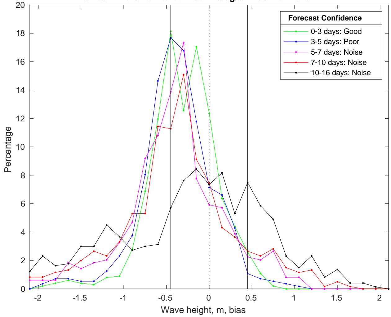
NDBC 46011 vs GFS Waves Bias Histogram: 30-Mar-2025
