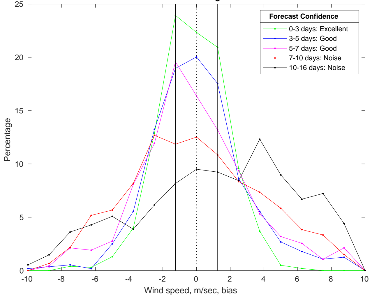
NDBC 46011 vs GFS Winds Bias Histogram: 30-Mar-2025
